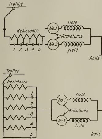
FIG. 1—SERIES AND PARALLEL STARTING RESISTANCE METHOD.
